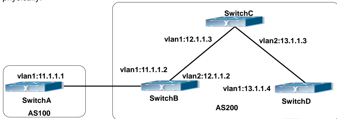
Fig 14-10 BGP Network Topological Map
