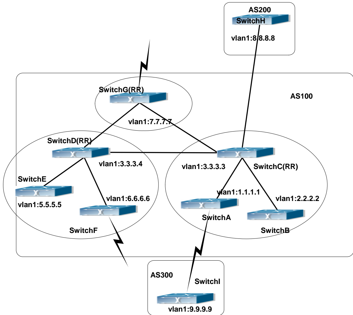
Fig 14-12 the Topological Map of Route Reflector
