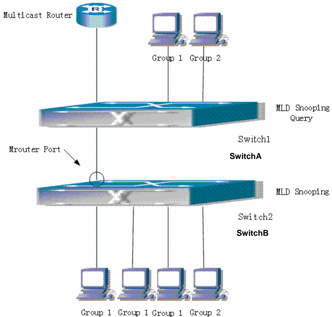
Fig 18-5 Switches as MLD Querier Function figure
