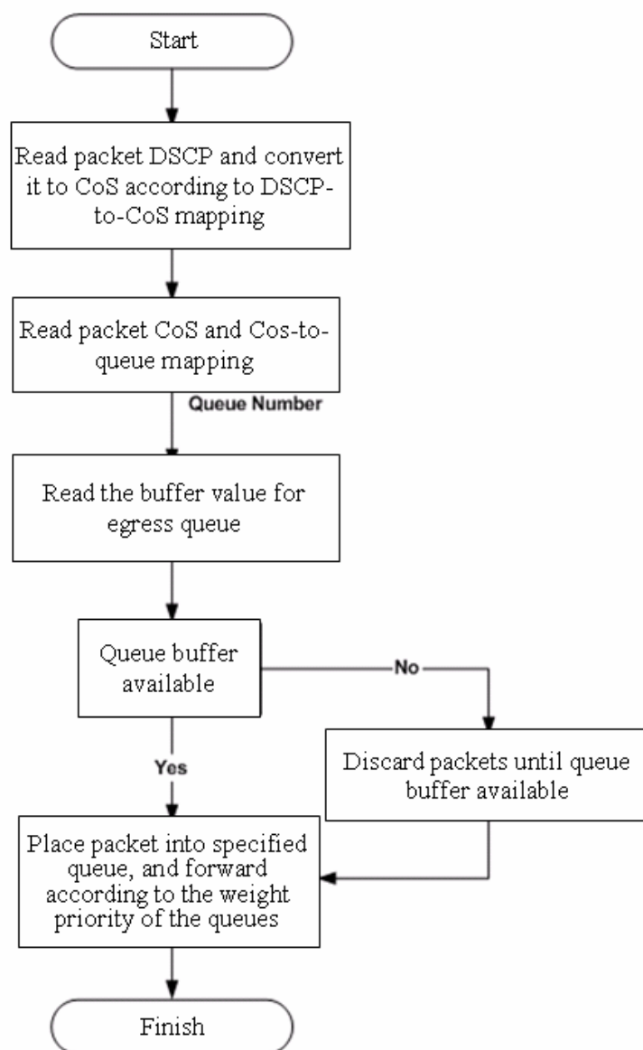
Fig 9-6Queuing and Scheduling process
