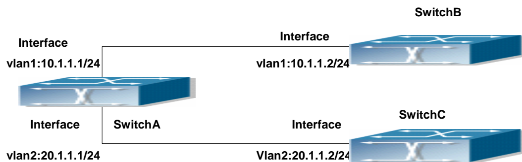
Fig 14-3 RIP example
