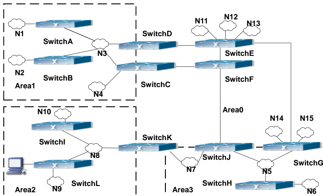
Fig 14-7 Typical complex OSPF autonomous system.
