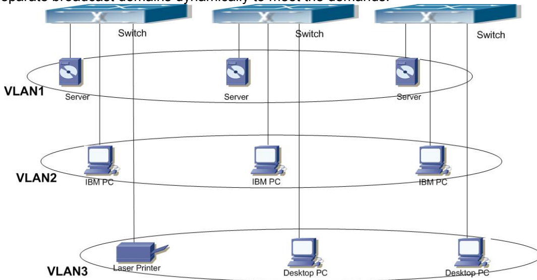
Fig 6-1 A VLAN network defined logically
