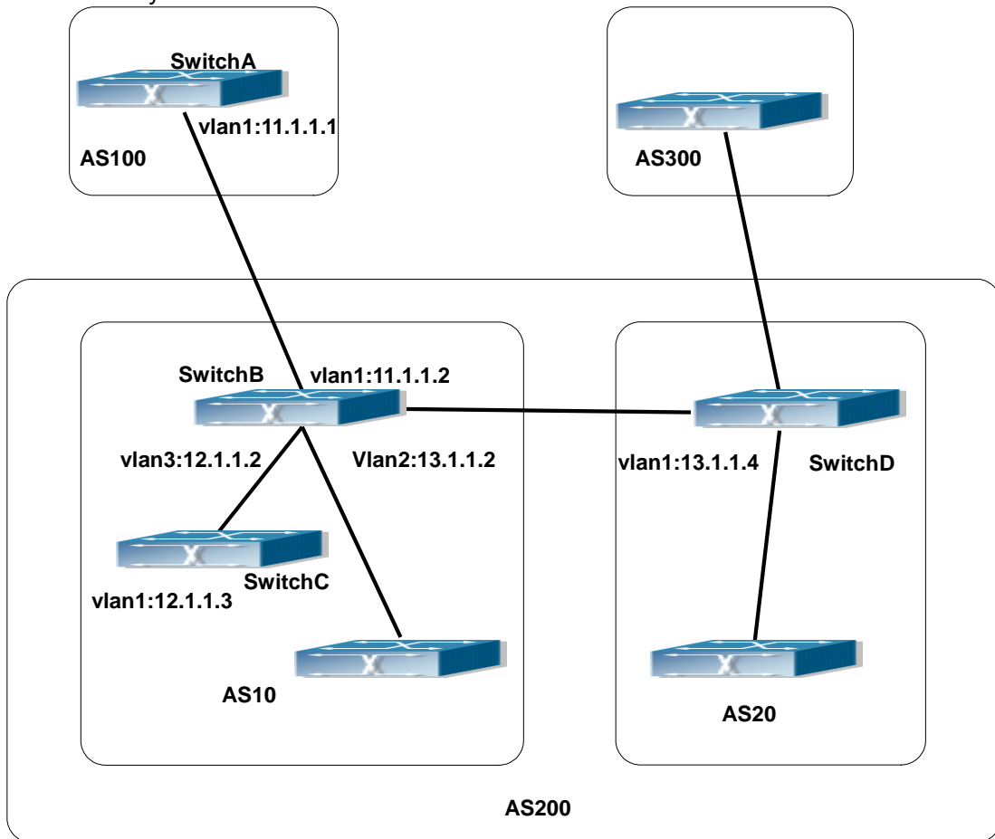
Fig 14-11 Confederation configuring topology
