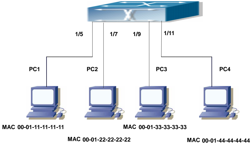
Fig 7-2 MAC Table typical configuration example
