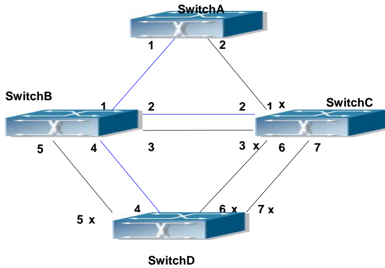
Fig 8-3 The Topology Of the Instance 0 after the MSTP Calculation
