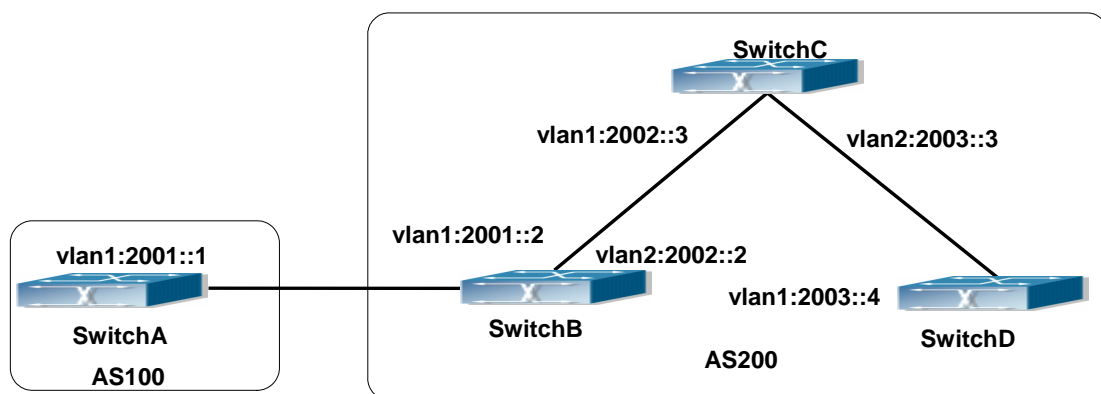
Fig 14-14 BGP Network Topological Map
