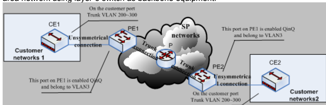
Fig 6-4 Dot1q-tunnel based Internetworking mode
