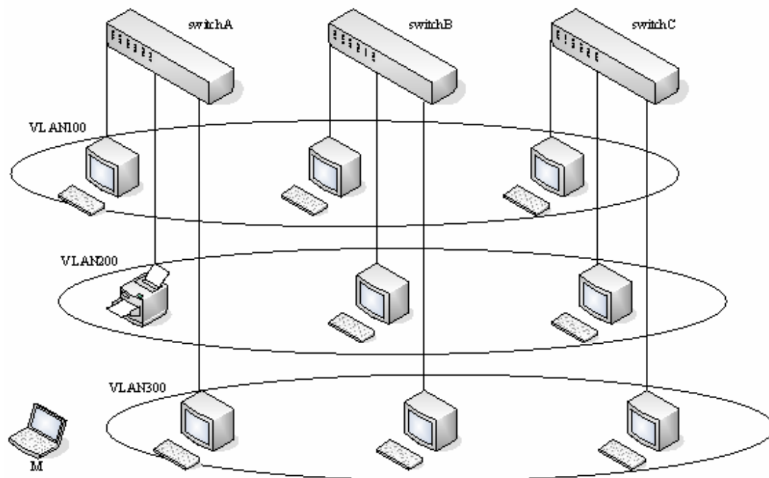
Figure 6-6 Typical topology application of dynamic VLAN
