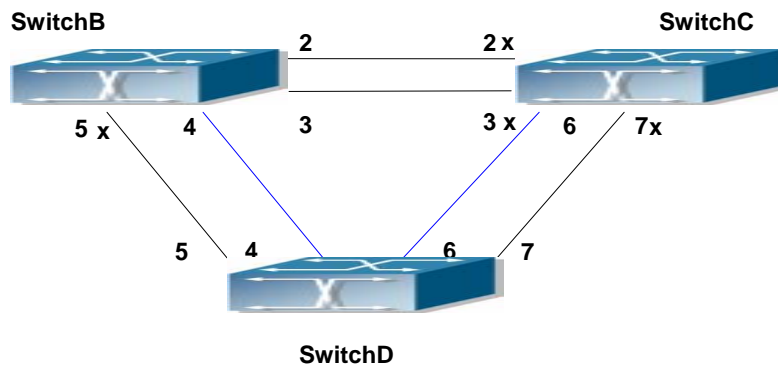
Fig 8-5 The Topology Of the Instance 4 after the MSTP Calculation
