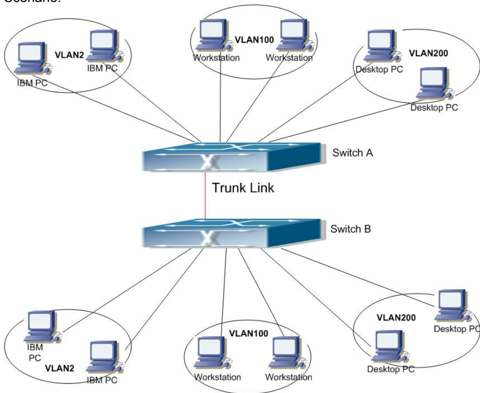
Fig 6-2 Typical VLAN Application Topology
