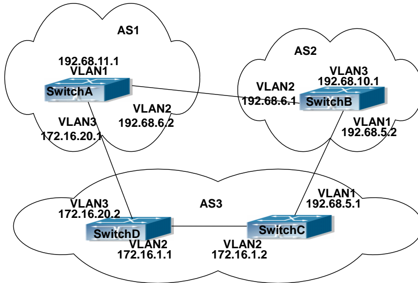
Fig 14-1 Policy routing Configuration
