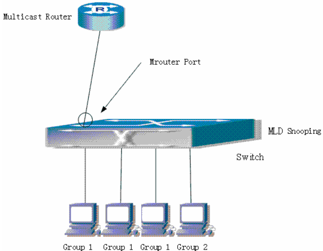
Fig 18-4 Switches as MLD Querier Function figure
