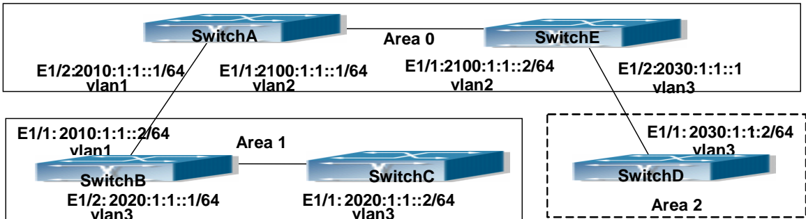
Fig 14-9 Network topology of OSPF autonomous system.
