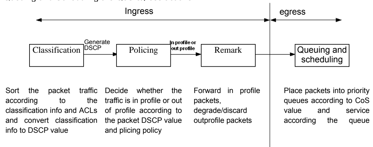
Fig 9-3 Basic QoS Model
