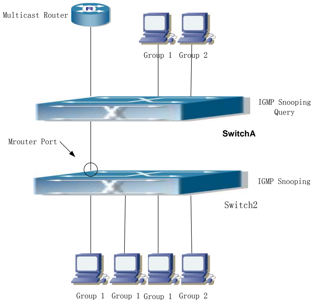
Fig 15-1 The switches as IGMP Queries
