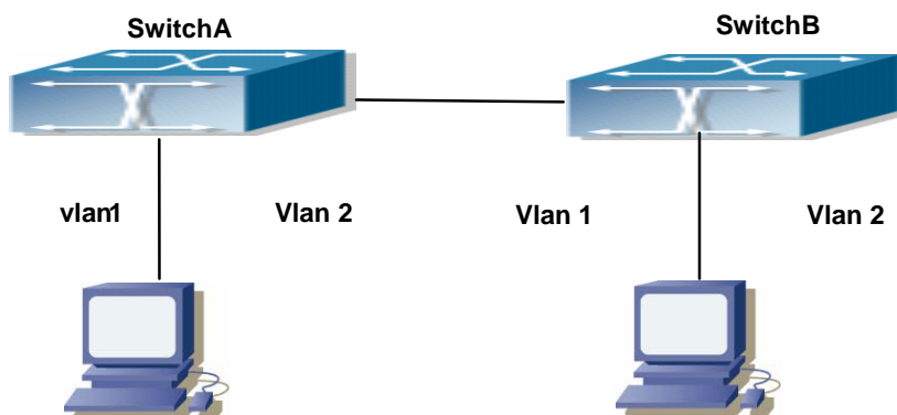
Fig 18-1PIM-DM Typical Environment
