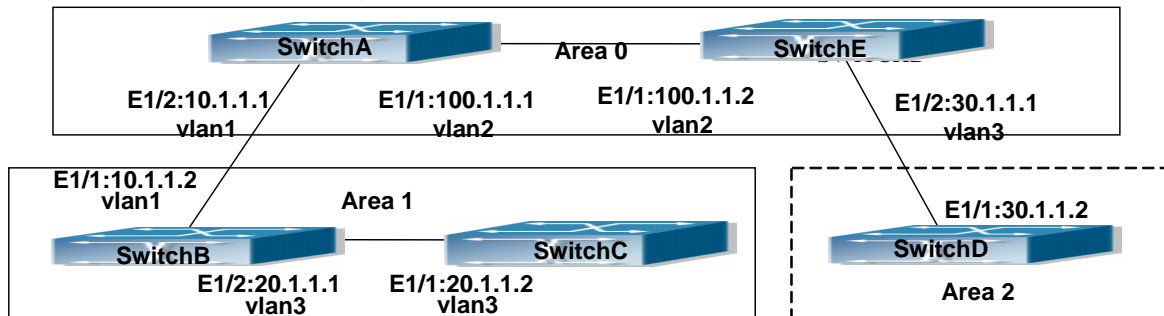
Fig 14-6 Network topology of OSPF autonomous system.
