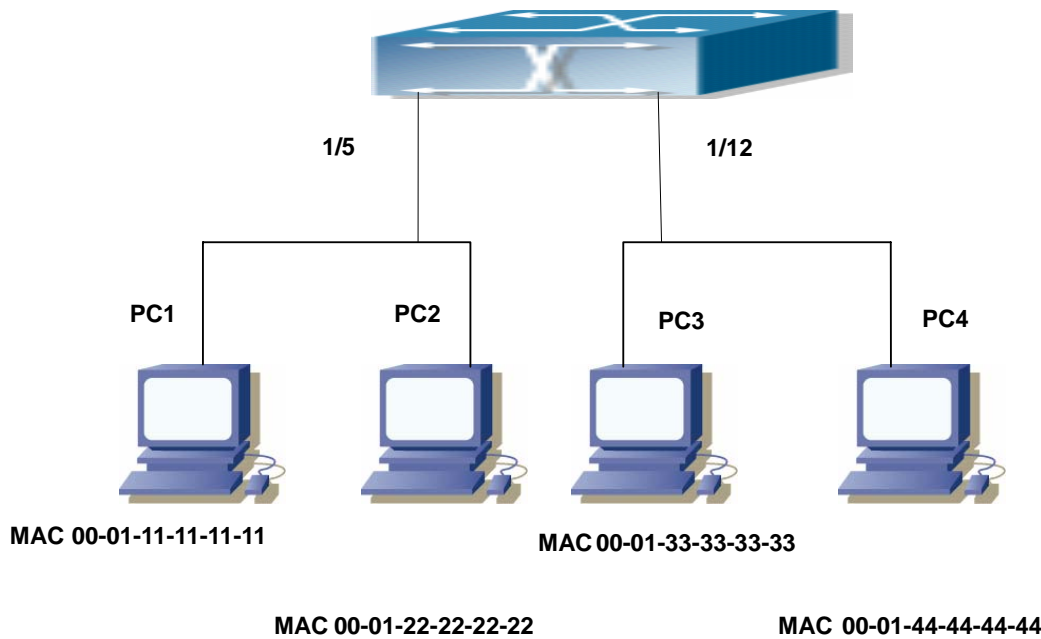
Fig 7-1 MAC Table dynamic learning
