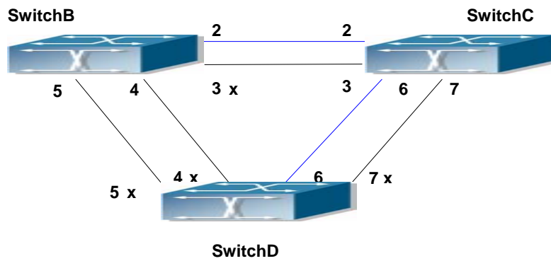
Fig 8-4 The Topology Of the Instance 3 after the MSTP Calculation
