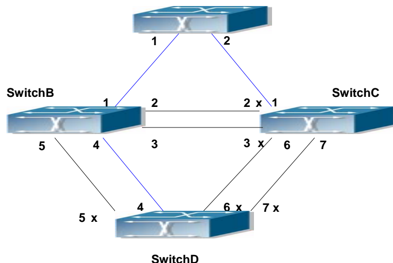
Fig 8-2Typical MSTP Application Scenario
