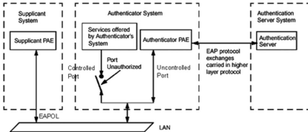
Fig 20-1 802.1x architecture
