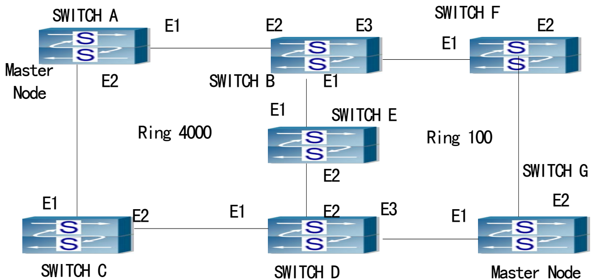
Fig 22-4 MRPP Scenario 3
