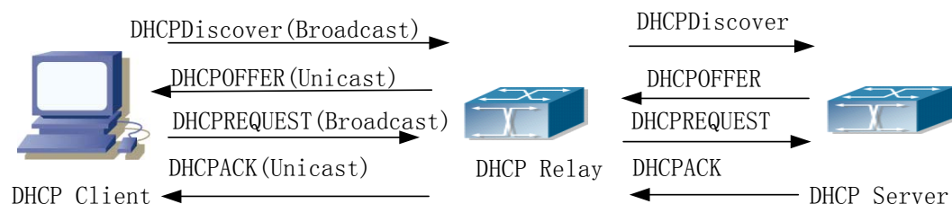
Fig 11-2 DHCP relay
