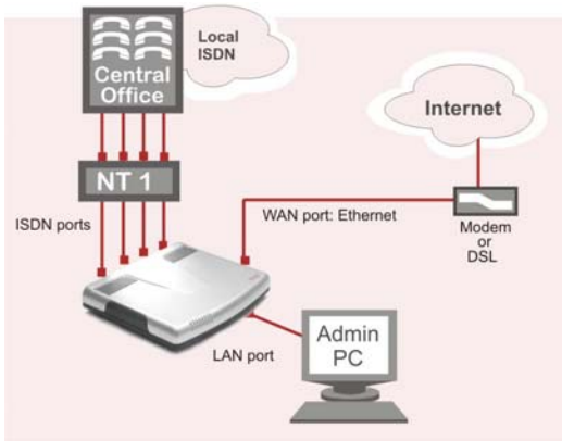
Fig. I-4: Configuration: Quadro used as Internet Access Router
