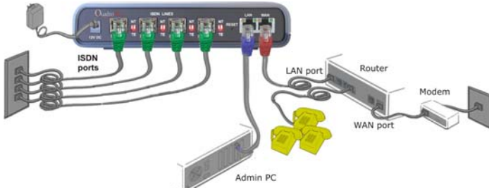
Fig. I- 5: Installation: Quadro4Li behind a router with IP phones on WAN
