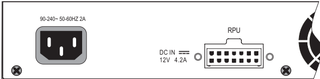
Figure 3-6 Power Receptacle
