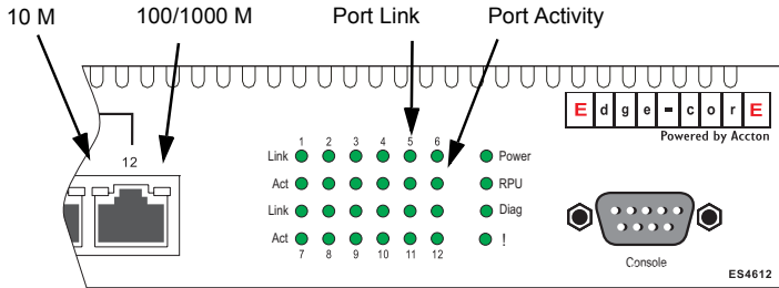
Figure 1-2 Port LEDs
