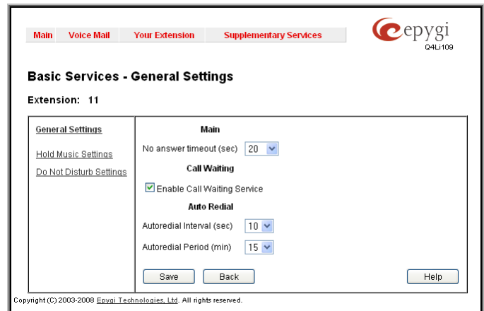
Fig. III-35 Basic Services – General Settings page
