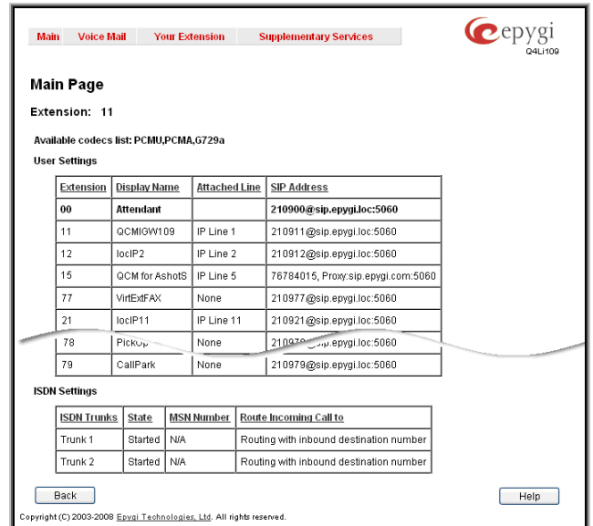
Fig.III-1 Extension's Main Page
