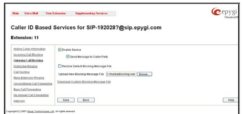
Fig. III-24 Outgoing Call Blocking page
