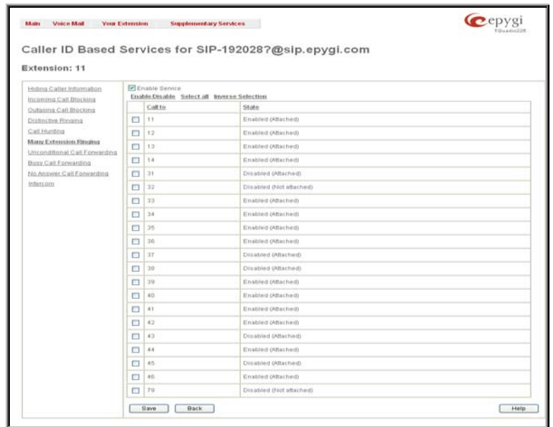
Fig. III-28 Many Extension Ringing page
