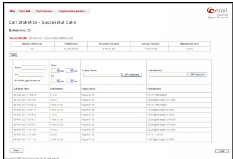
Fig. III-12 Extension's Call Statistics page
