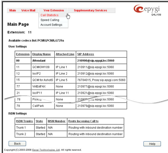
Fig.III-10 Your Extension menu in Dynamo theme
