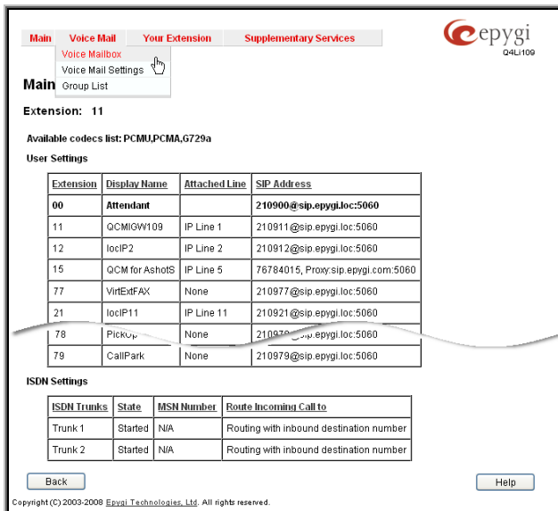
Fig. III-2 Voice Mail menu in Dynamo Theme
