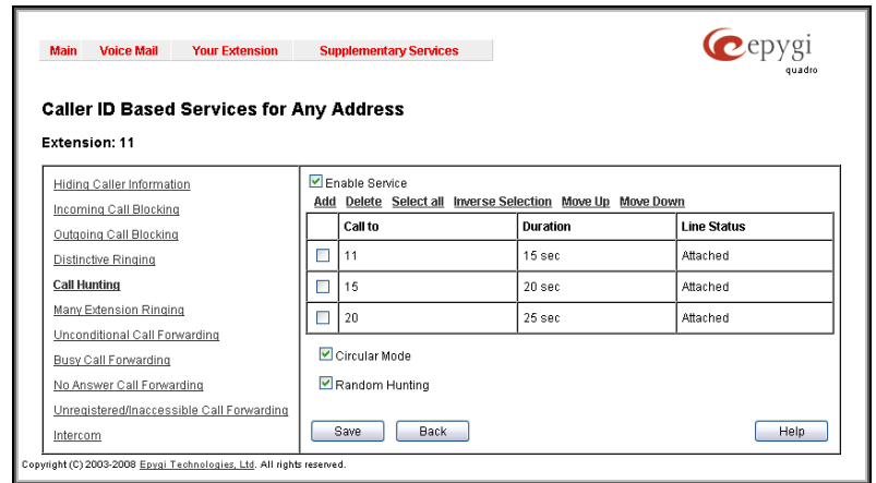
Fig. III-26 Call Hunting page
